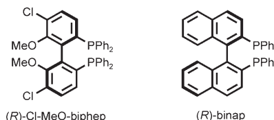
Scheme 1. Reactions of 1-phenyl-2-propynyl acetate ( 1a ) with N -methylaniline in the presence of a catalytic amount of copper trifluoromethanesulfonate benzene complex and ( R )-Cl-MeO-biphep or ( R )-binap.
